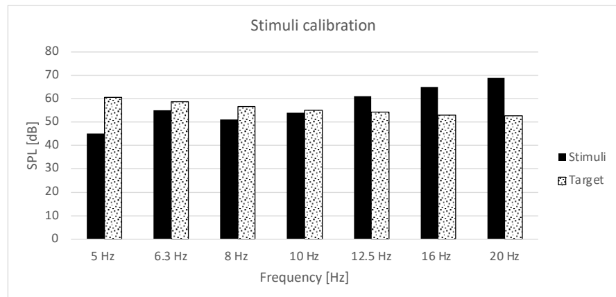
Figure 2. The target level of the wind turbine noise and the resulting stimuli after calibration.
